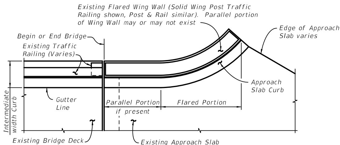
PARTIAL PLAN VIEW OF EXISTING BRIDGE WITH INTERMEDIATE WIDTH CURBS, FLARED WING WALLS AND FLARED INTEGRAL APPROACH SLAB CURBS - USE INDEX 521-483, SCHEME 3
