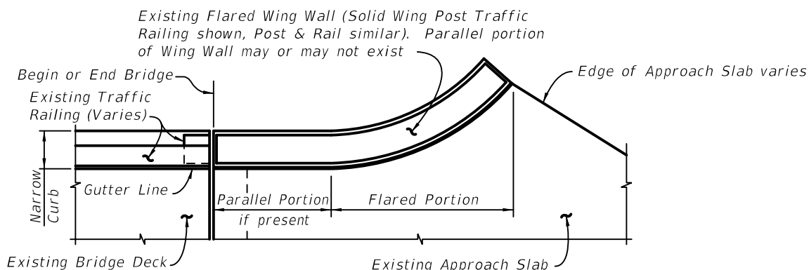
PARTIAL PLAN VIEW OF EXISTING BRIDGE WITH NARROW CURBS AND FLARED WING WALLS - USE INDEX 521-481, SCHEME 3
