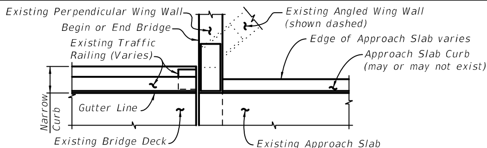
PARTIAL PLAN VIEW OF EXISTING BRIDGE WITH NARROW CURBS AND PERPENDICULAR OR ANGLED WING WALLS - USE INDEX 521-481, SCHEME 1
