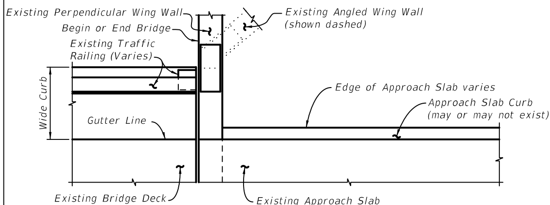
PARTIAL PLAN VIEW OF EXISTING BRIDGE WITH WIDE CURBS AND PERPENDICULAR OR ANGLED WING WALLS - USE INDEX 521-482, SCHEME 1
