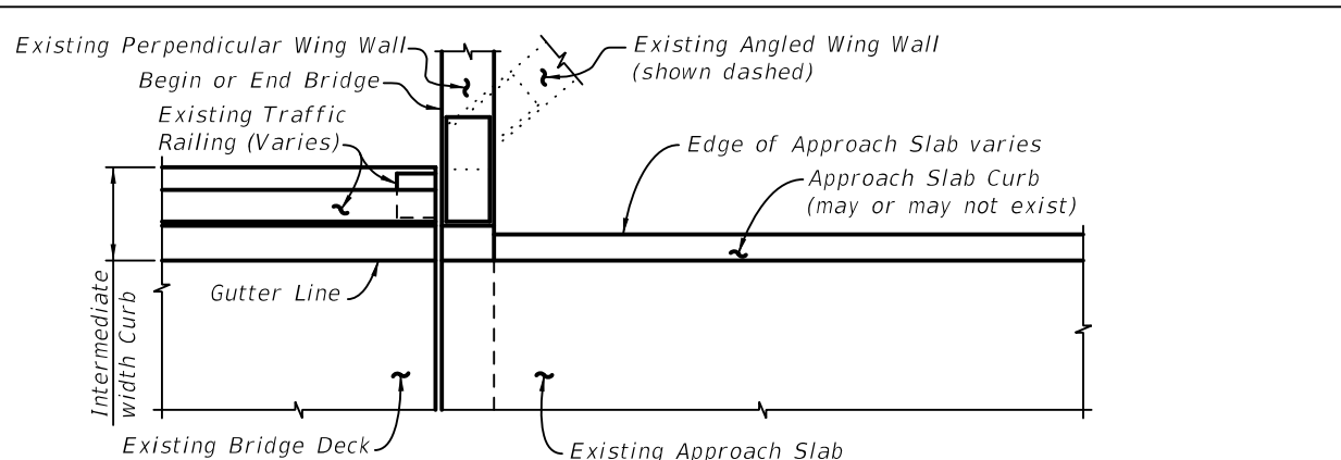
PARTIAL PLAN VIEW OF EXISTING BRIDGE WITH INTERMEDIATE WIDTH CURBS AND PERPENDICULAR OR ANGLED WING WALLS - USE INDEX 521-483, SCHEME 1
