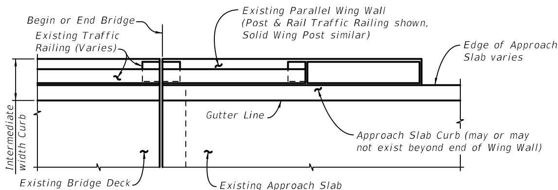
PARTIAL PLAN VIEW OF EXISTING BRIDGE WITH INTERMEDIATE WIDTH CURBS, PARALLEL WING WALLS AND PARALLEL INTEGRAL APPROACH SLAB CURBS - USE INDEX 521-483, SCHEME 2
