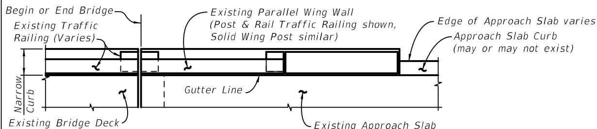
PARTIAL PLAN VIEW OF EXISTING BRIDGE WITH NARROW CURBS AND PARALLEL WING WALLS - USE INDEX 521-481, SCHEME 2
