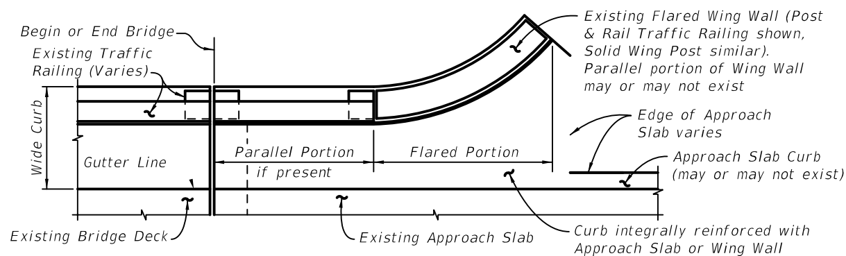
PARTIAL PLAN VIEW OF EXISTING BRIDGE WITH WIDE CURBS, FLARED WING WALLS AND PARALLEL INTEGRALLY REINFORCED APPROACH SLAB CURBS - USE INDEX 521-482, SCHEME 2
