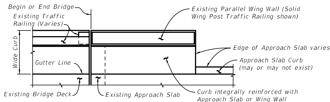
PARTIAL PLAN VIEW OF EXISTING BRIDGE WITH WIDE CURBS, PARALLEL WING WALLS AND INTEGRALLY REINFORCED APPROACH SLAB CURBS - USE INDEX 521-482, SCHEME 2
