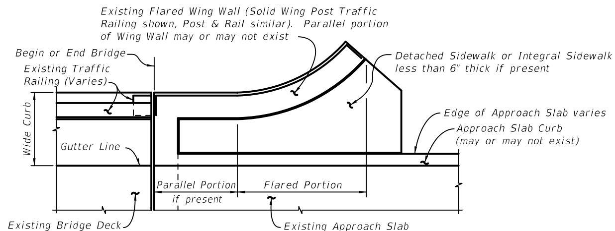
PARTIAL PLAN VIEW OF EXISTING BRIDGE WITH WIDE CURBS, FLARED WING WALLS AND APPROACH SLABS WITH DETACHED SIDEWALKS OR SIDEWALKS LESS THAN 6" THICK - USE INDEX 521-482, SCHEME 5
