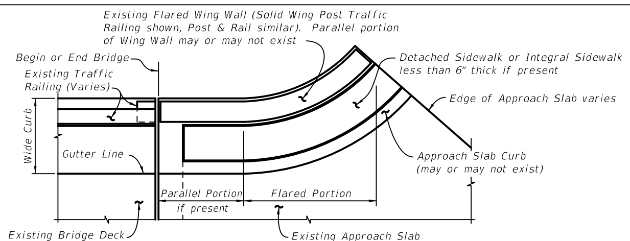
PARTIAL PLAN VIEW OF EXISTING BRIDGE WITH WIDE CURBS, FLARED WING WALLS AND APPROACH SLABS WITH DETACHED SIDEWALKS OR SIDEWALKS LESS THAN 6" THICK - USE INDEX 521-482, SCHEME 4
