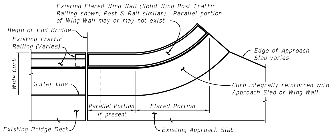
PARTIAL PLAN VIEW OF EXISTING BRIDGE WITH WIDE CURBS, FLARED WING WALLS AND FLARED INTEGRALLY REINFORCED APPROACH SLAB CURBS - USE INDEX 521-482, SCHEME 3
