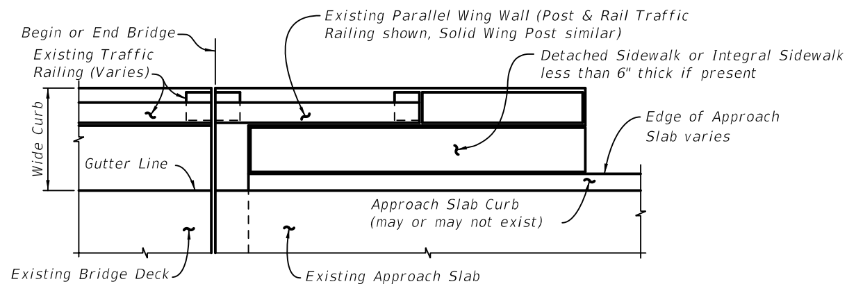
PARTIAL PLAN VIEW OF EXISTING BRIDGE WITH WIDE CURBS, PARALLEL WING WALLS AND APPROACH SLABS WITH DETACHED SIDEWALKS OR SIDEWALKS LESS THAN 6" THICK - USE INDEX 521-482, SCHEME 5
