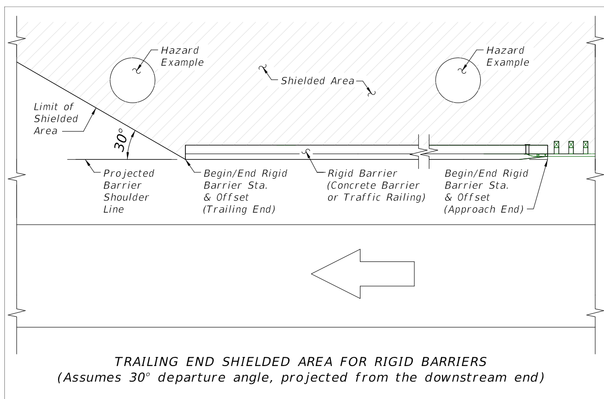
Figure 1: Trailing End Barrier Placement
