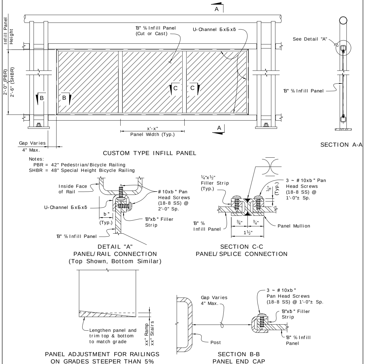
STEEL PEDESTRIAN/ BICYCLE RAILING CUSTOM TYPE INFILL PANEL DETAILS
