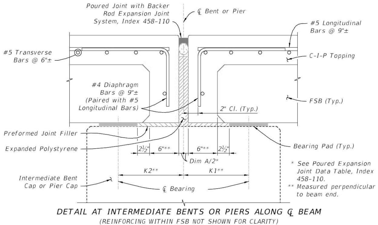
Figure 8a Detail at Intermediate Bents/Piers—Option 1 (Open Joint)
