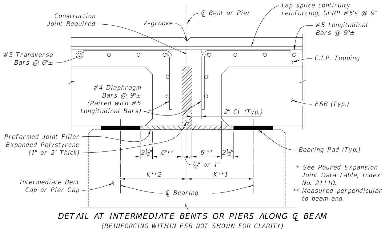
Figure 8b Detail at Intermediate Bents/Piers–Option 2 (Link-Slab)
