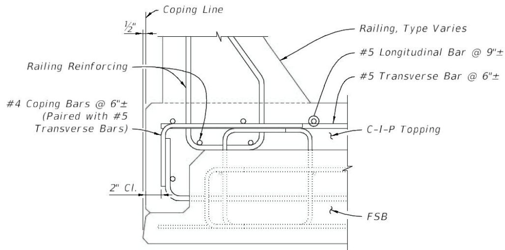
DETAIL AT COPINGS
