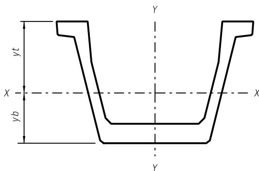
FLORIDA-U BEAM (FUB) SECTION (FUB-63 INDEX 450-263 SHOWN, OTHERS SIMILAR)
