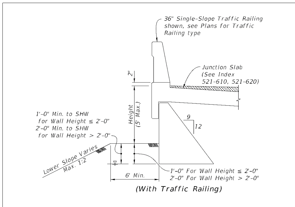
Figure 3 Minimum Toe Berm Width for Overall Stability - Scheme 3
