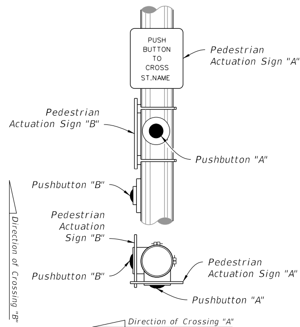
DETAIL "A"
