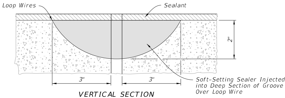
VERTICAL SECTION
