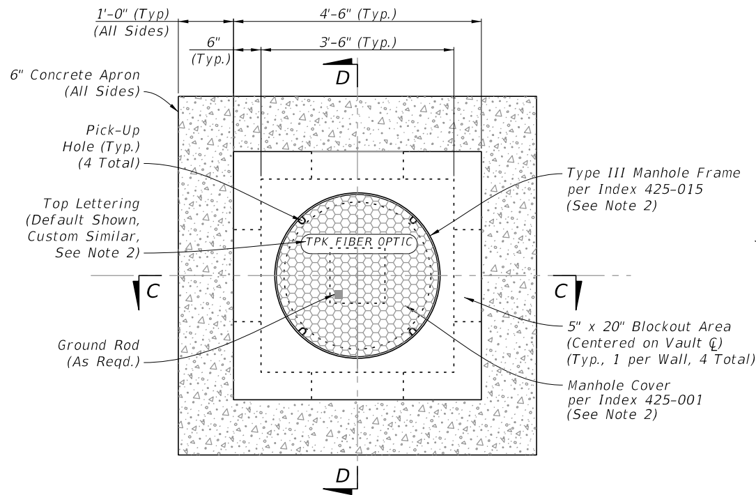
PLAN VIEW (Symmetrical About CL)
