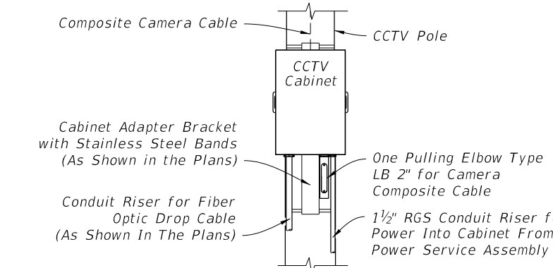
FRONT VIEW DETAIL "E"
