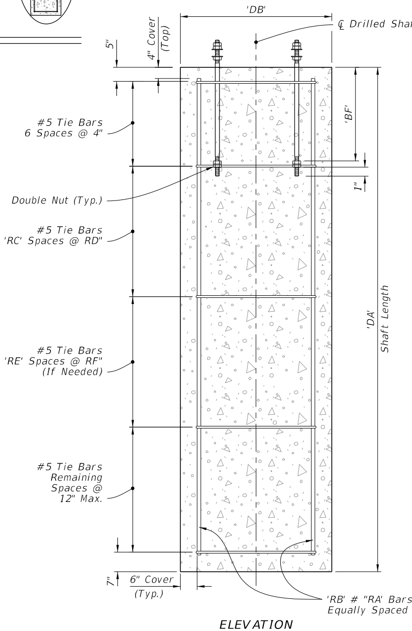
FOUNDATION
