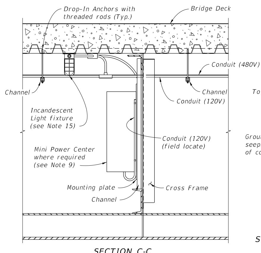
SECTION C-C
