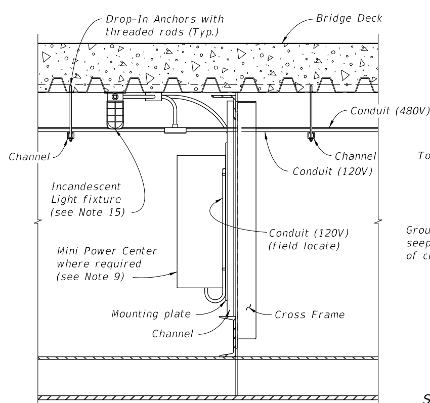
SECTION C-C
