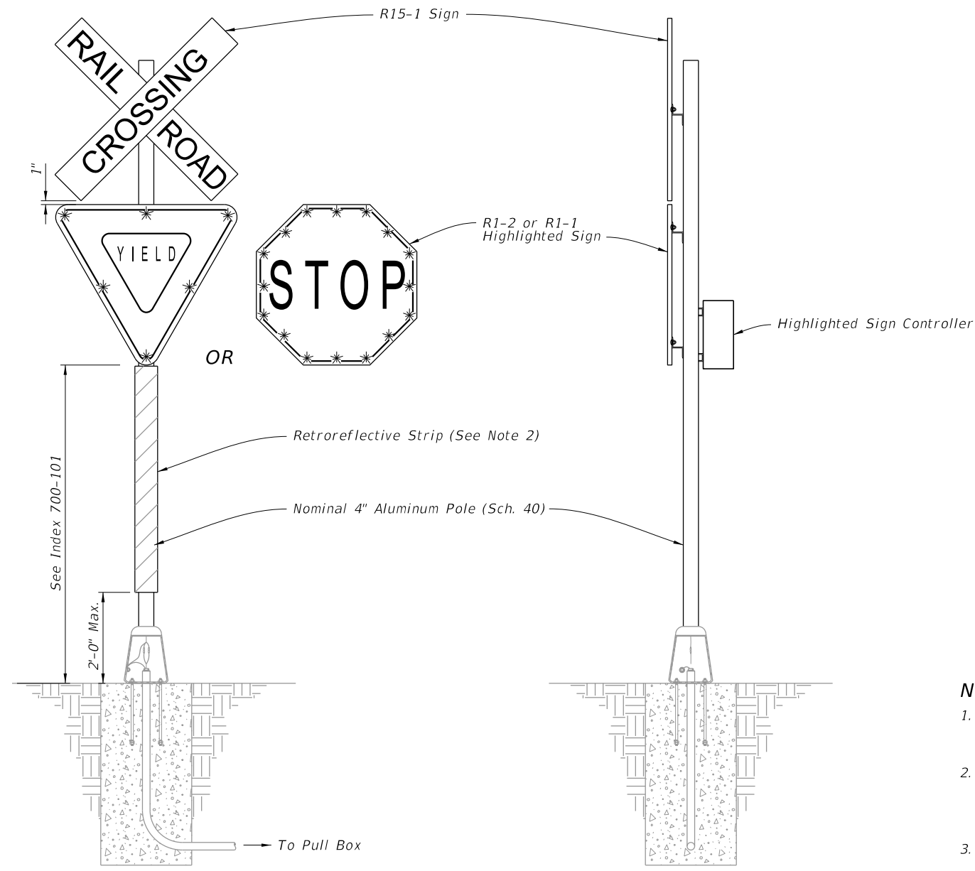
FRONT ELEVATION
