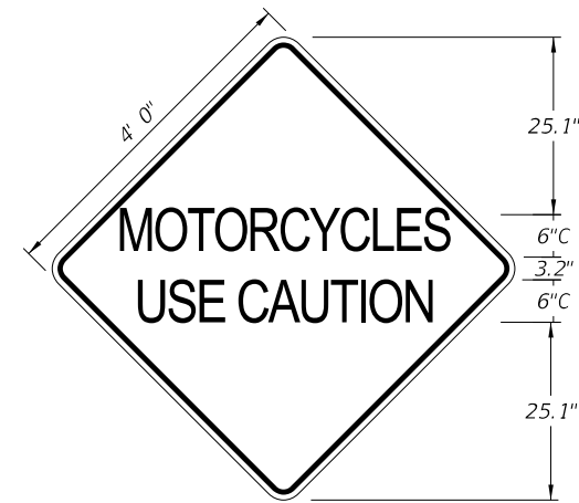
TTC-020B-25 4'-0" x 4'-0" 1.5" Radii \frac{3}{4} " Border 6" Series C Legend Pink Background Black Legend and Border
