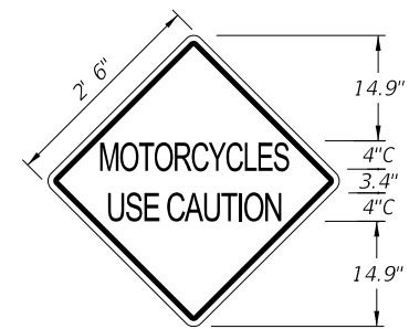
TTC-020-25 2'-6" x 2'-6" 1.5" Radii \frac{3}{4} " Border 4" Series C Legend Pink Background Black Legend and Border
