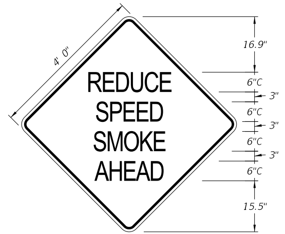
TTC-019A-25 4'-0" x 4'-0" 3" Radii \frac{3}{4} " Border 6" Series C Legend Pink Background Black Legend and Border
