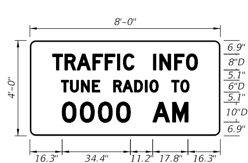
FTP-423-25 8'-0" X 4'-0" 3" Radii \frac{3}{4} " Border 6", 8" and 10" Series D Legend Blue Background White Legend and Border
