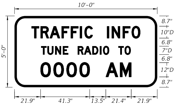
FTP-423A-25 10'-0" X 5'-0" 9" Radii 2" Border 7", 10" and 12" Series D Legend Blue Background White Legend and Border
