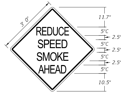
TTC-019-25 3'-0" x 3'-0" 1.5" Radii \frac{3}{4} " Border 5" Series C Legend Pink Background Black Legend and Border
