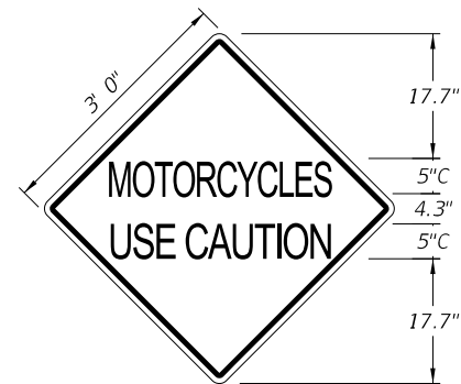
TTC-020A-25 3'-0" x 3'-0" 1.5" Radii \frac{3}{4} " Border 5" Series C Legend Pink Background Black Legend and Border
