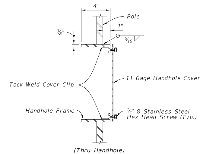
HANDHOLE FRAME
