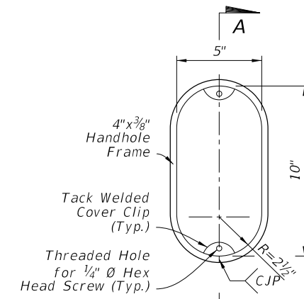
HANDHOLE FRAME
