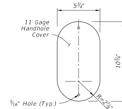
COVER
