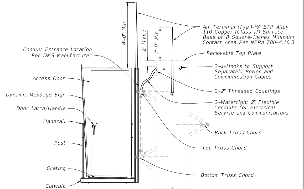
DETAIL "A"
