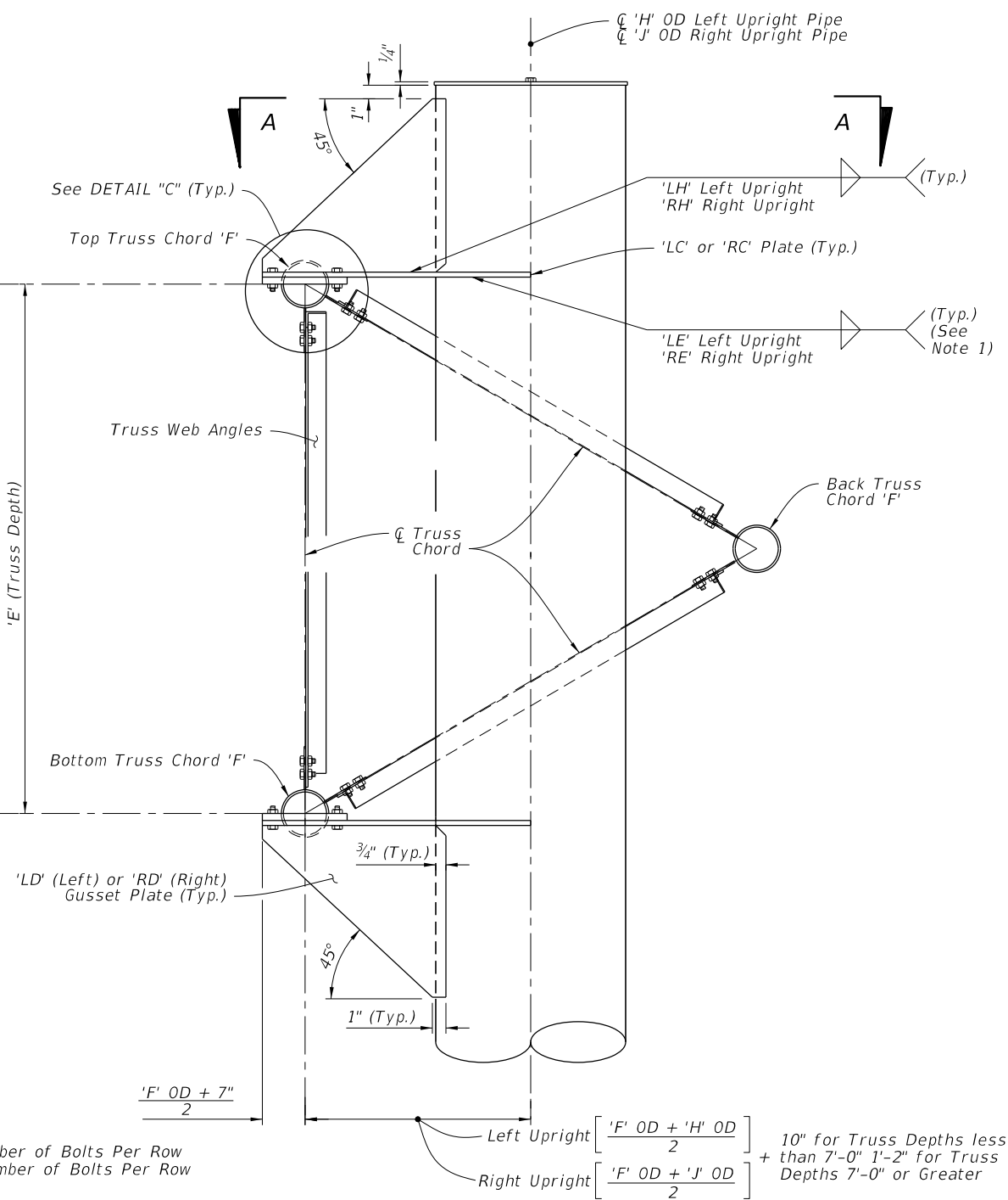
SIDE ELEVATION
