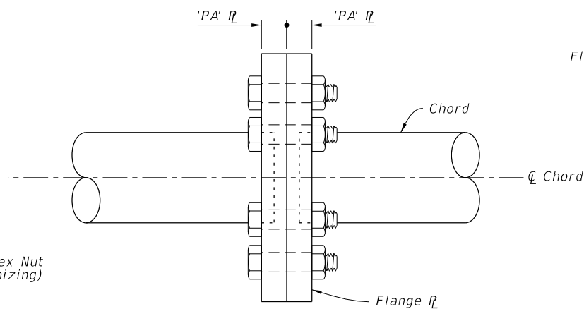
FRONT ELEVATION
