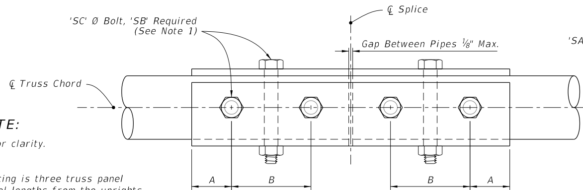
FRONT ELEVATION
