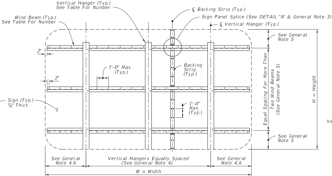
BACK ELEVATION
