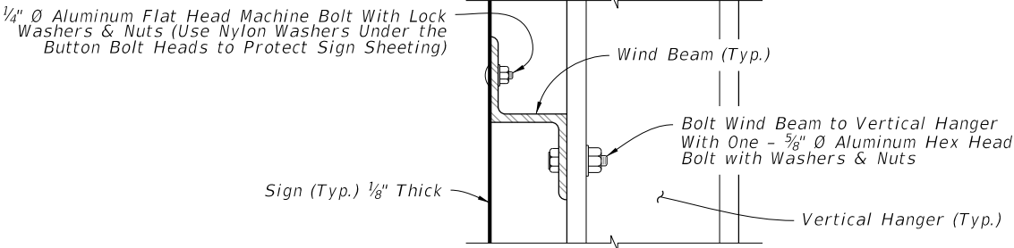
DETAIL "B"
