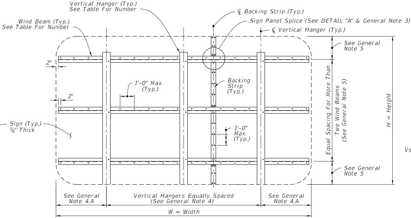
BACK ELEVATION
