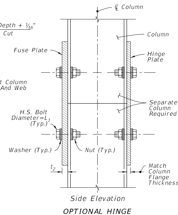
DETAIL "B"
