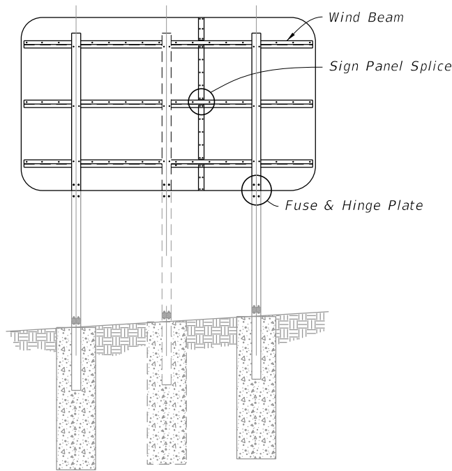
BACK ELEVATION
