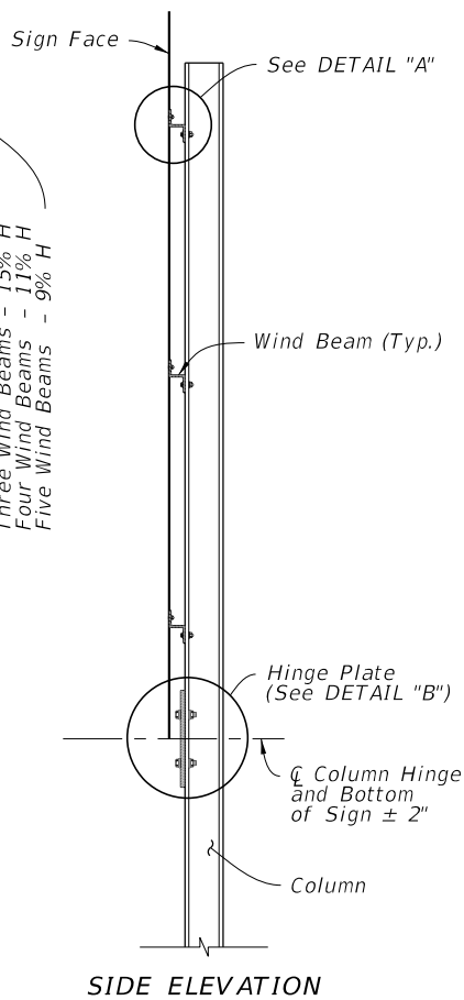
SIDE ELEVATION
