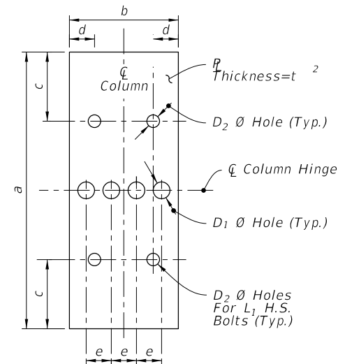
FUSE PLATE
