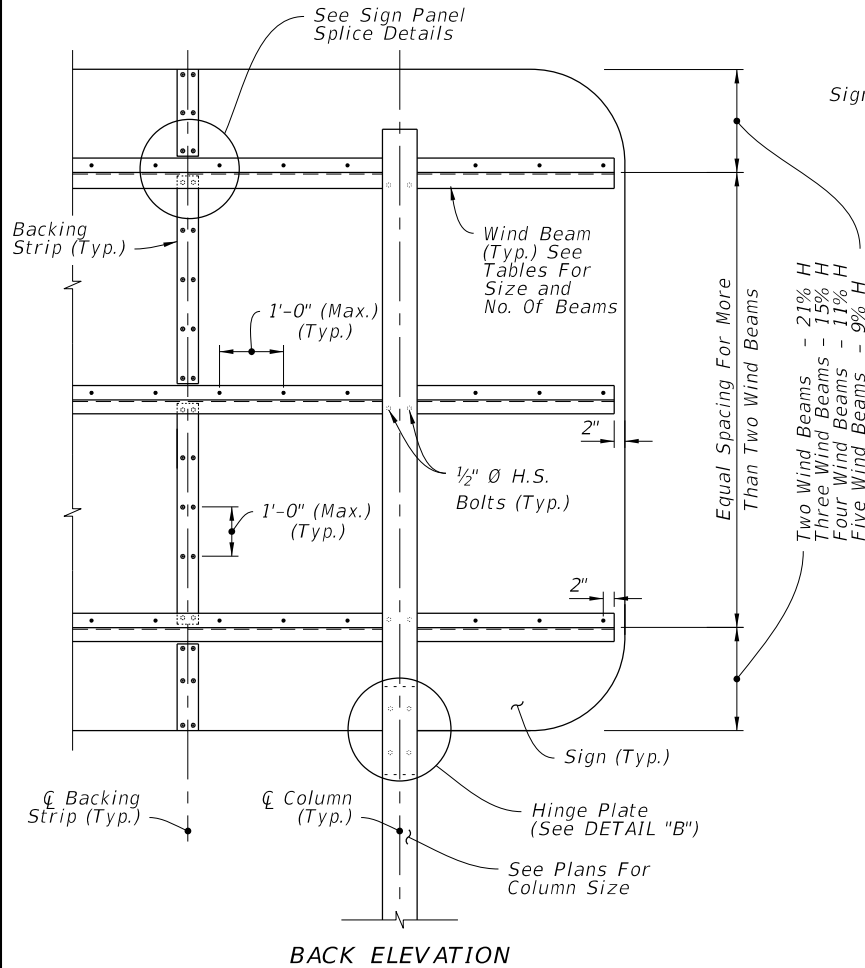
BACK ELEVATION
