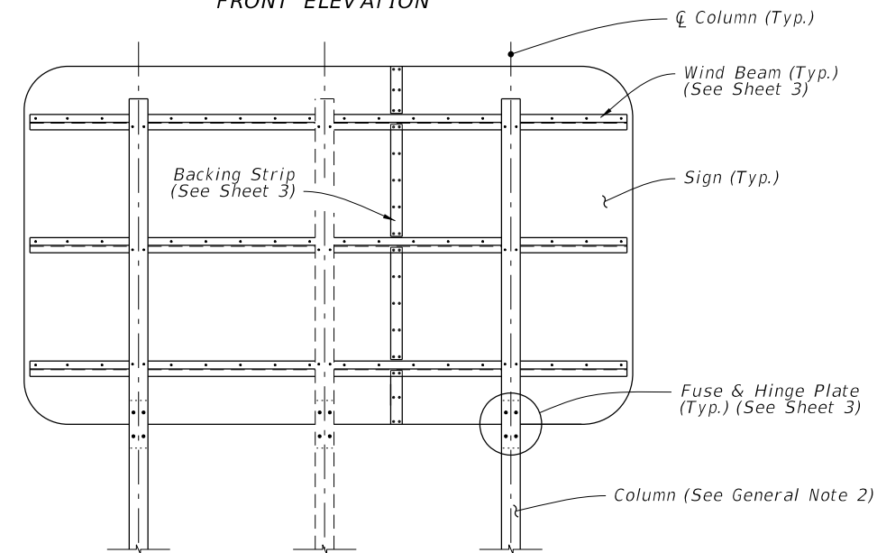
BACK ELEVATION
