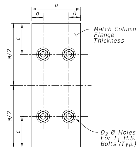
HINGE PLATE
