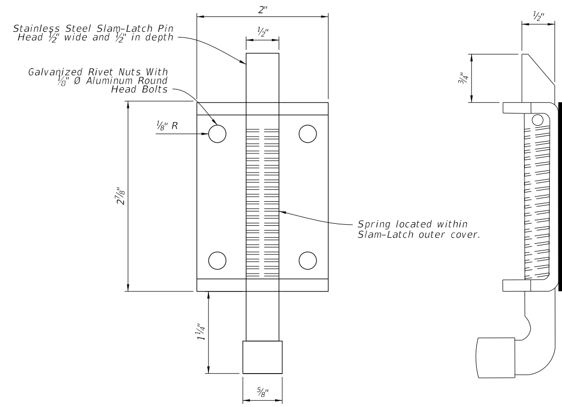
Stainless Steel Slam-Latch
