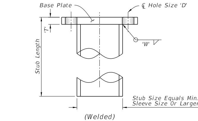
STUB DETAIL
