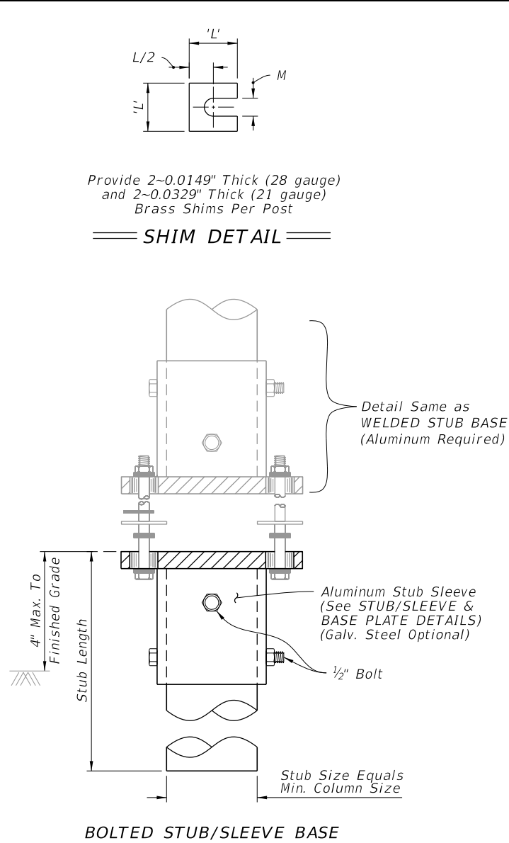
DETAIL 'A'
