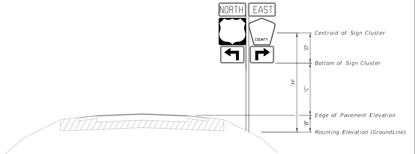
TYPICAL SECTION
