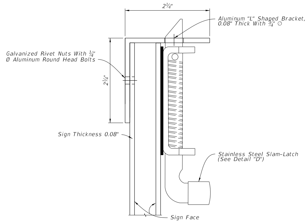
DETAIL "A"
