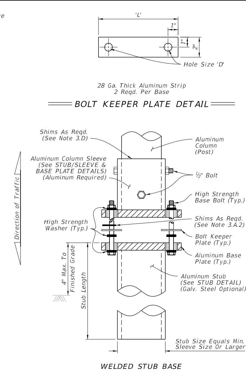
DETAIL 'A'
