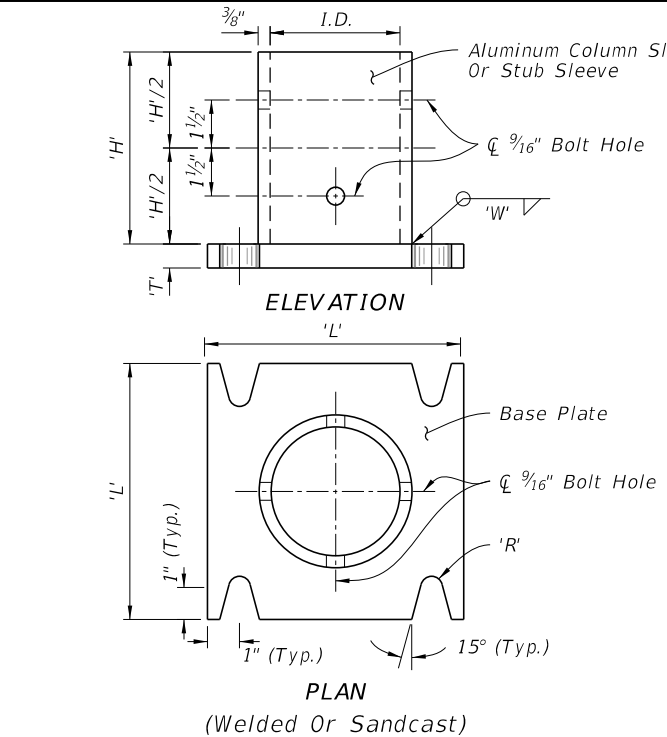
STUB/SLEEVE & BASE PLATE DETAILS
