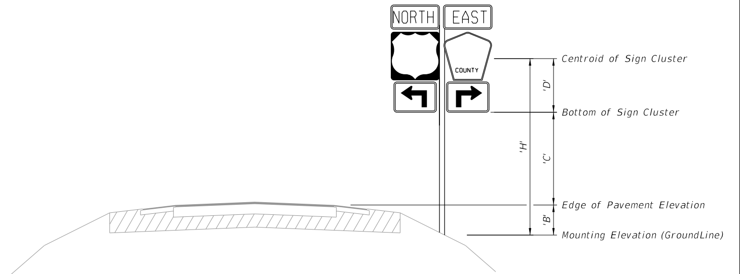
TYPICAL SECTION
