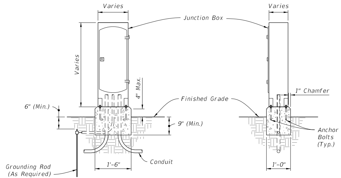
FRONT ELEVATION
