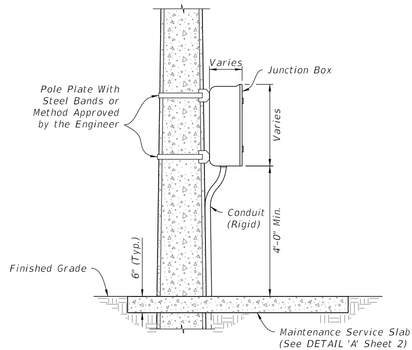
SIDE ELEVATION
