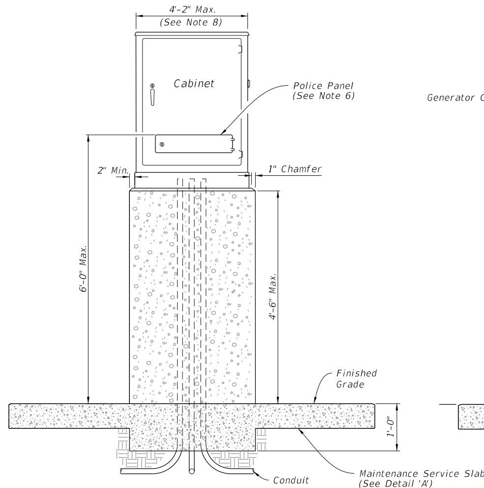
FRONT ELEVATION
