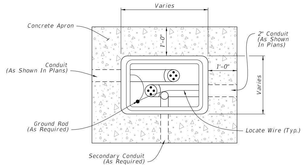
PLAN
