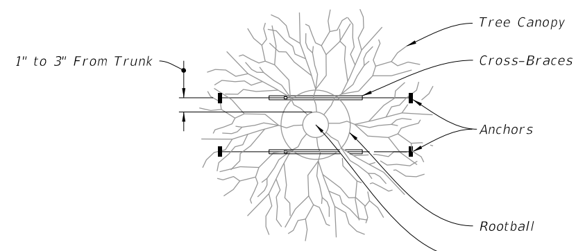
PLAN
