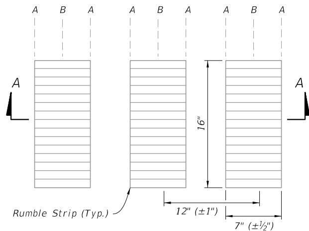
RUMBLE STRIP DETAILS
