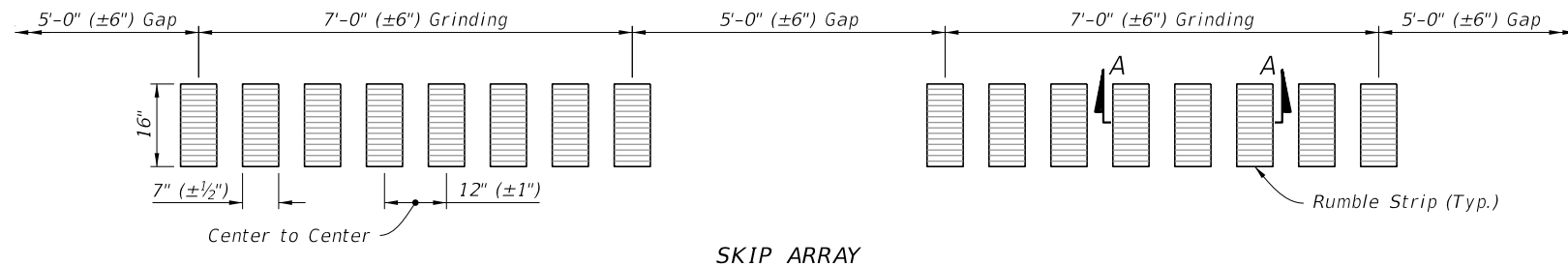
SKIP ARRAY
