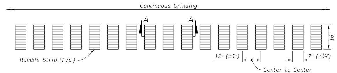
CONTINUOUS ARRAY
