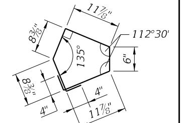
BAR P5 (45° Corner) Bar Length = 4'-6 1/2"
