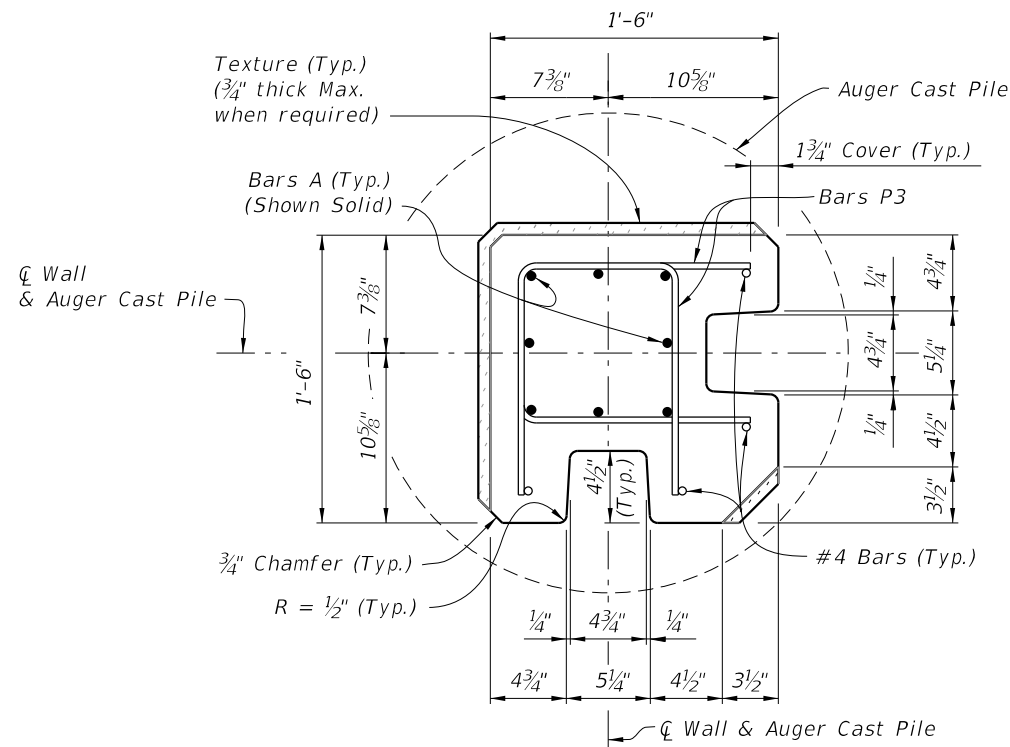
SECTION H-H
