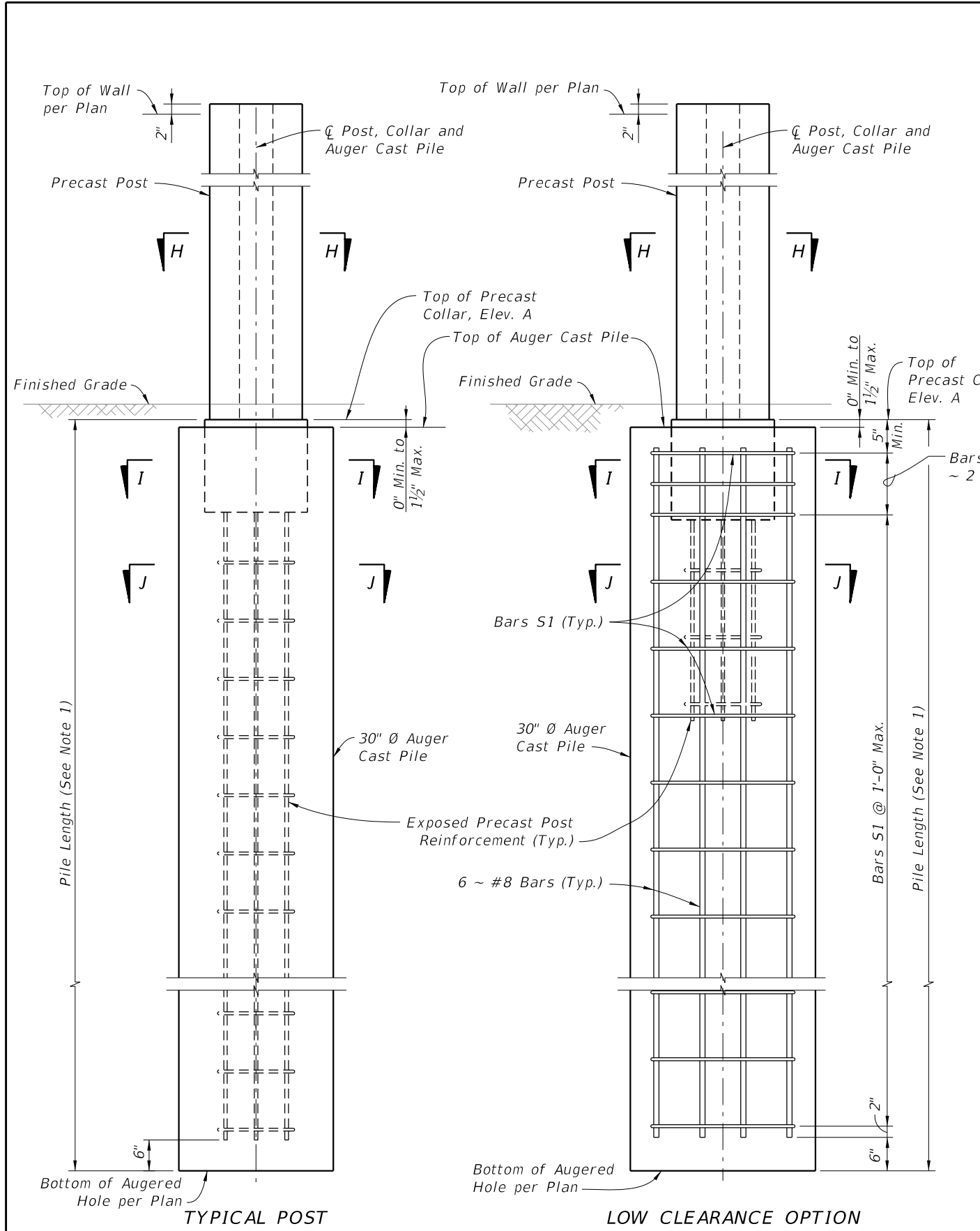
STANDARD POST PLACEMENT IN AUGER CAST PILE (Standard Post Shown, 45° and 90° Corner Posts Similar)
