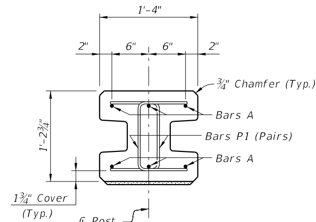
TYPICAL POST SECTION (H Section)
