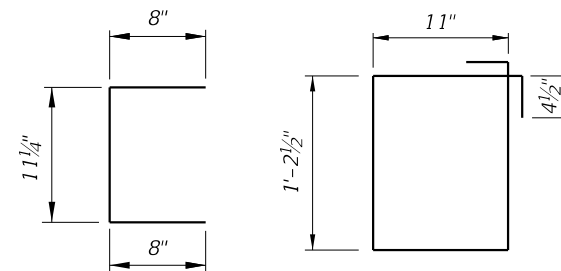
BAR BENDING DETAILS
