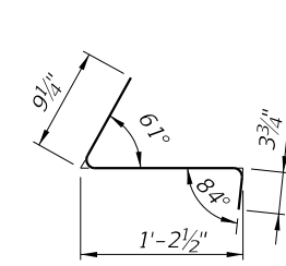
BAR P4 (45° Corner) Bar Length = 2'-3 1/2"
