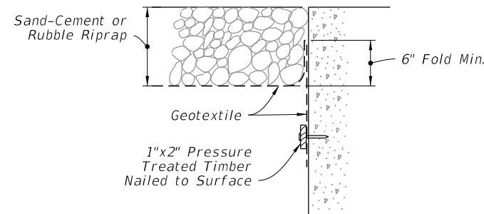
NAILED OPTION
