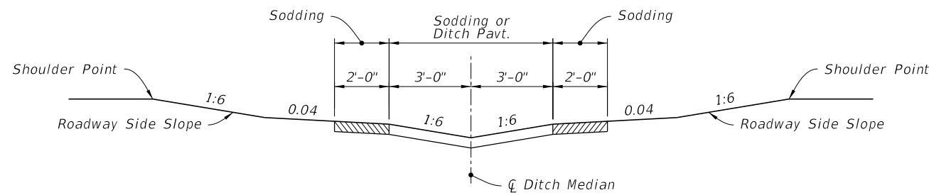
SWALED MEDIAN (No Weep Holes)
