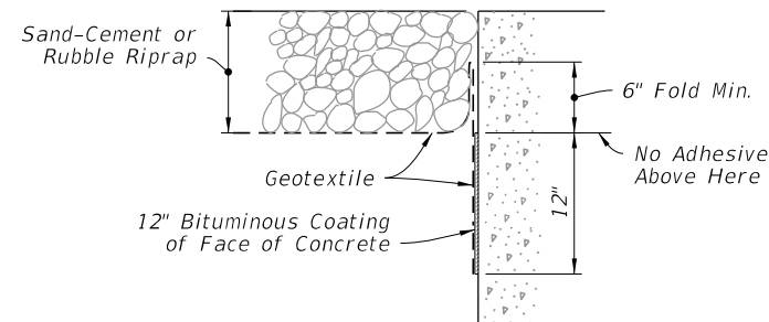
BONDED OPTION
