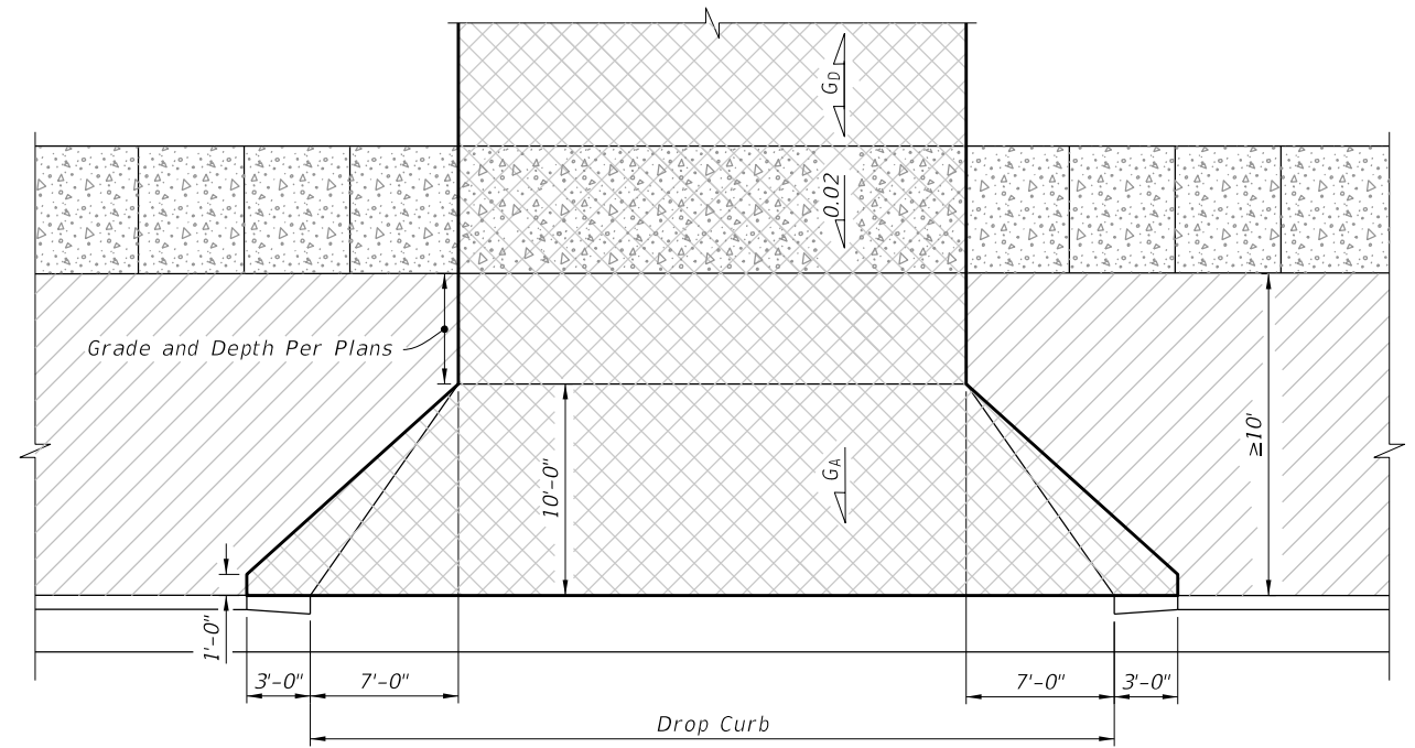
WITHOUT SIDEWALK OR UTILITY STRIP \geq 10' WIDE
