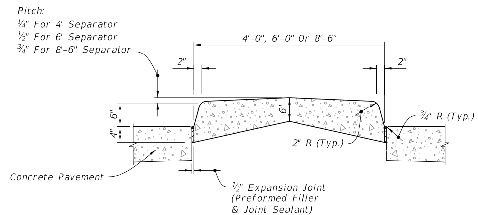
TRANSVERSE SECTION
