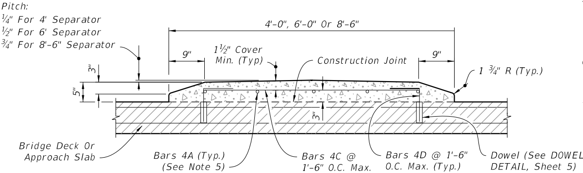
TRANSVERSE SECTION
