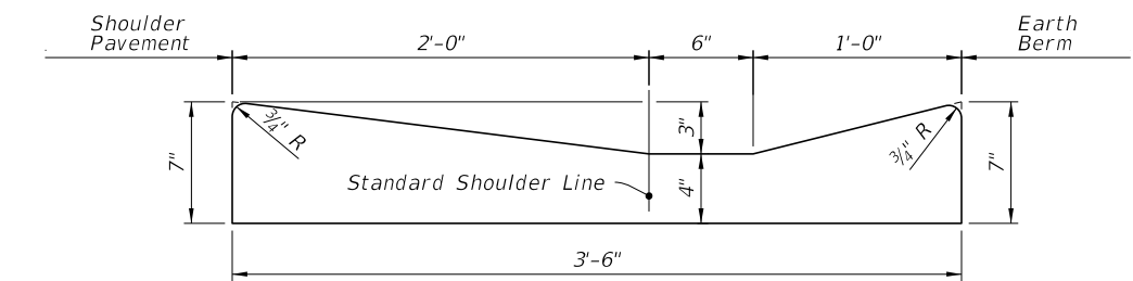
SHOULDER GUTTER
