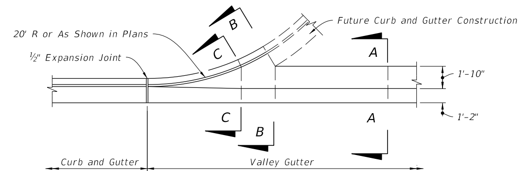
PLAN VIEW
