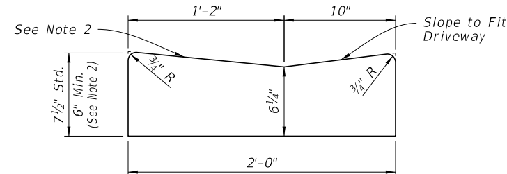
DROP CURB
