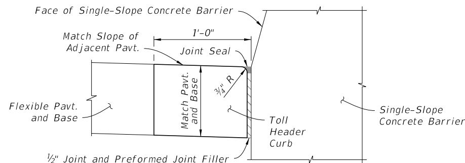
DROP CURB
