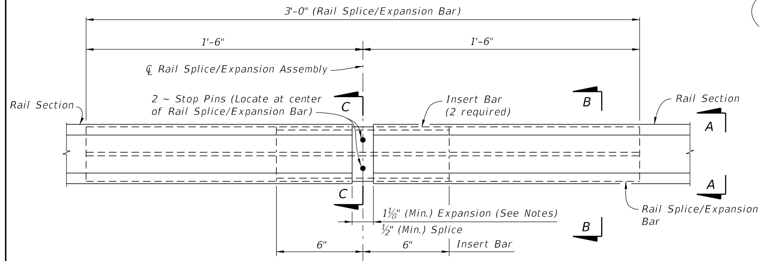
RAIL SPLICE/EXPANSION ASSEMBLY DETAIL
