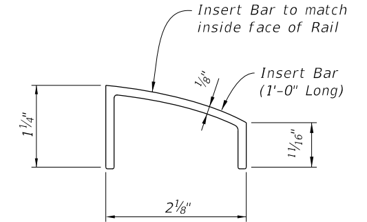
INSERT BAR DETAIL (TYPE 1)
