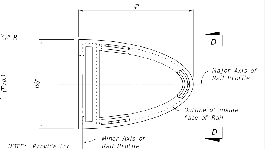
RAIL END CAP DETAIL
