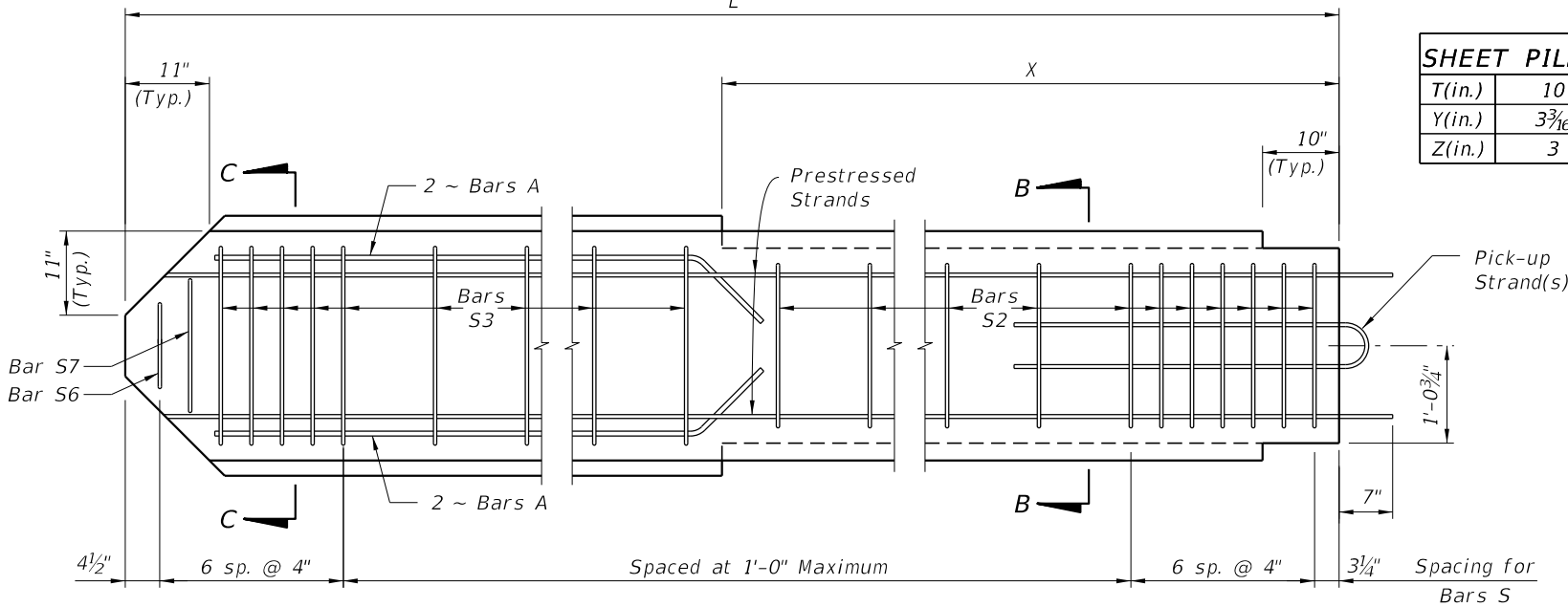
STARTER PILE
