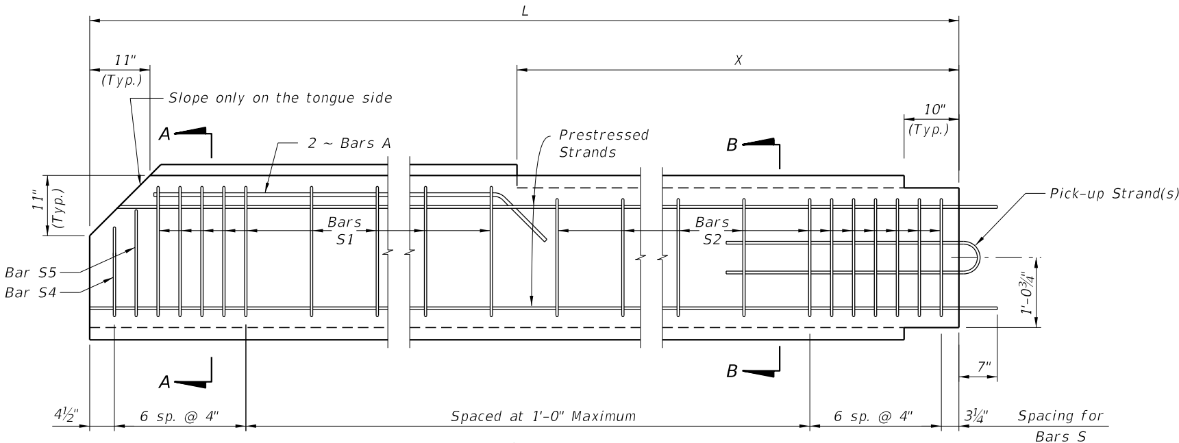
TYPICAL PILE
