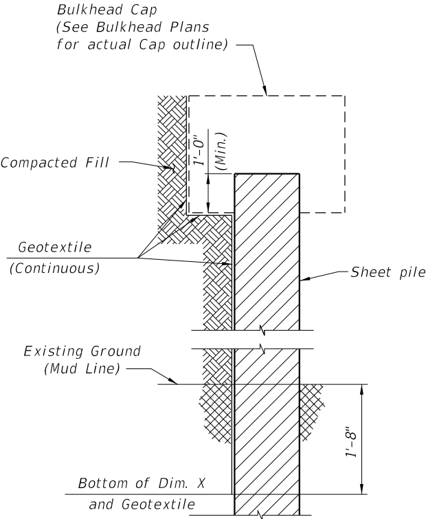
SECTION THRU BULKHEAD (Showing Geotextile)
