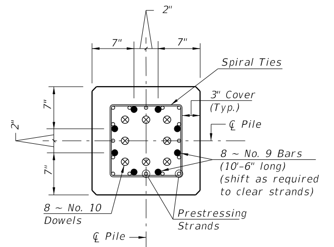
SECTION F-F
