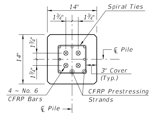
SECTION E-E
