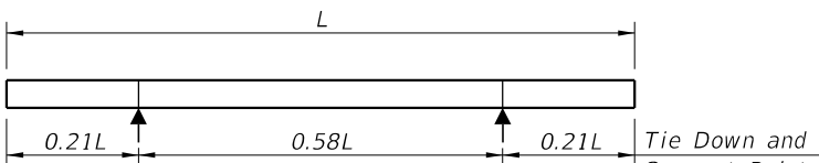
2-POINT SUPPORT
