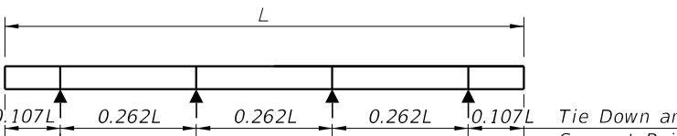
4-POINT SUPPORT
