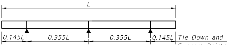
3-POINT SUPPORT
