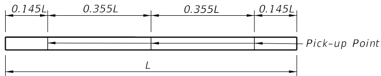
3-POINT PICK-UP
