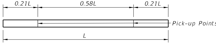
2-POINT PICK-UP
