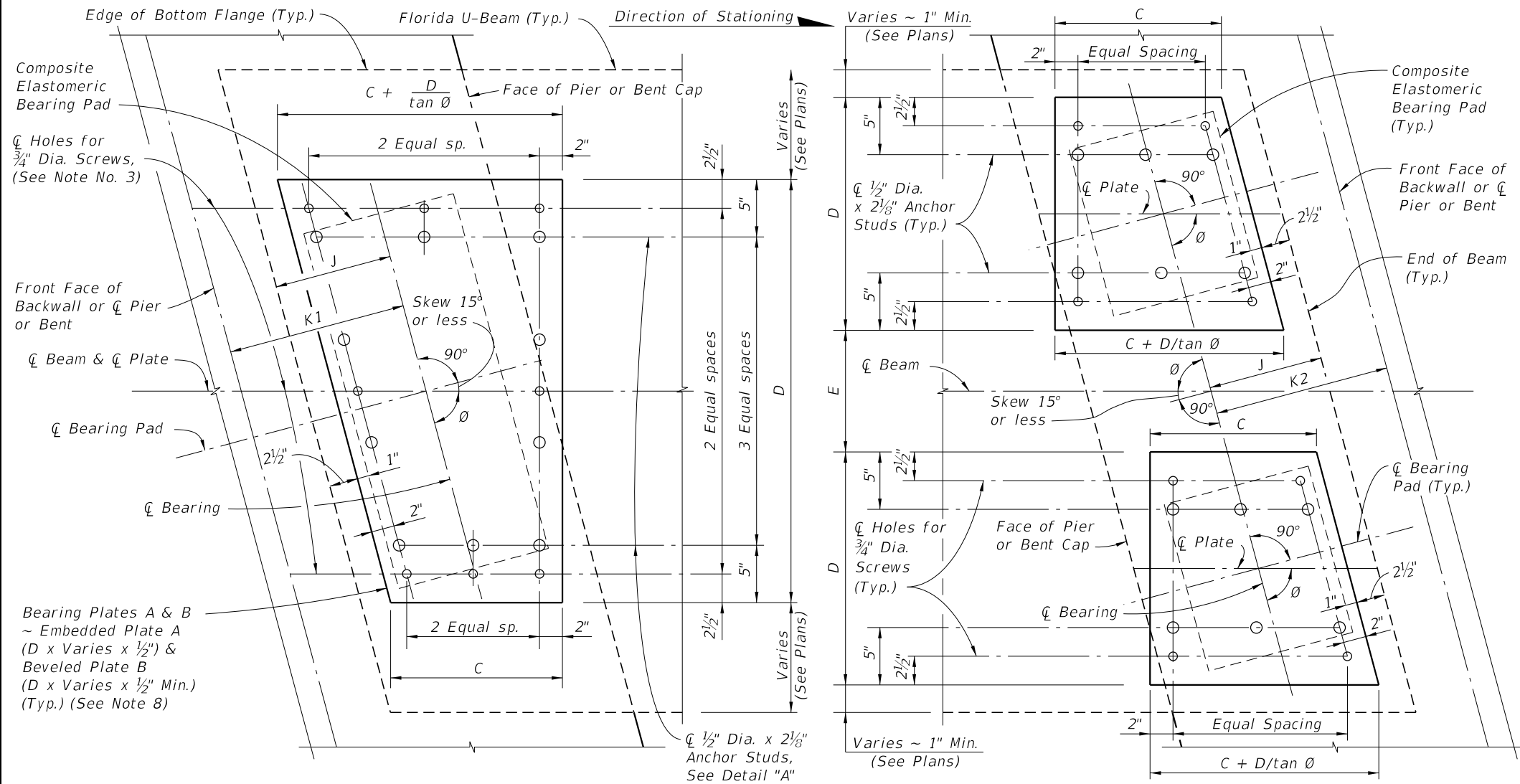
PLAN VIEW OF TYPICAL SINGLE BEARING
