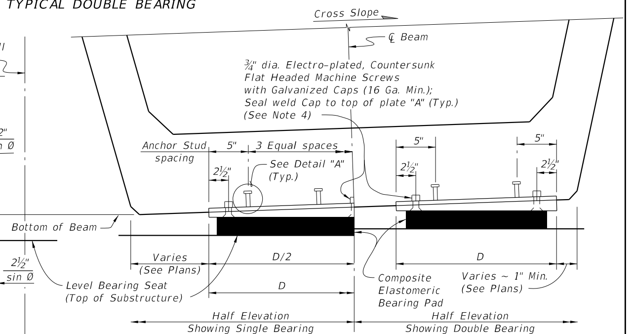
END ELEVATION (Positive Cross Slope shown, Negative Cross Slope similar)
