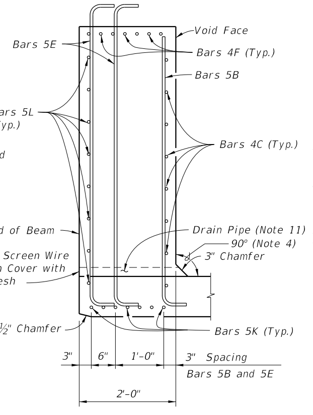
SECTION C-C
