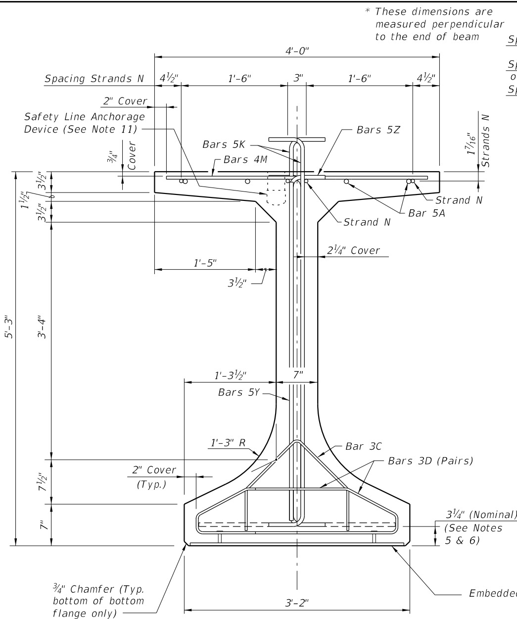
END VIEW
