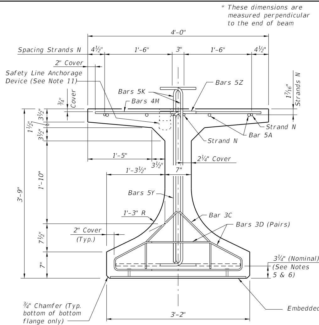
END VIEW
