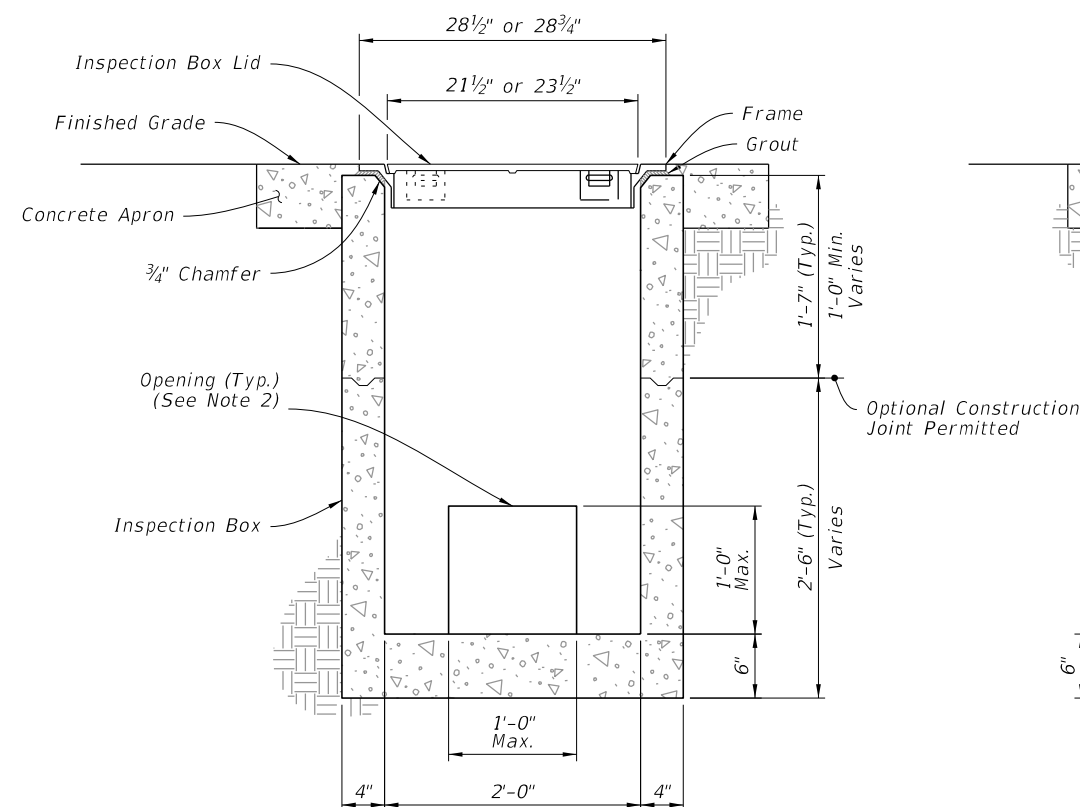
ELEVATION (FRONT VIEW)
