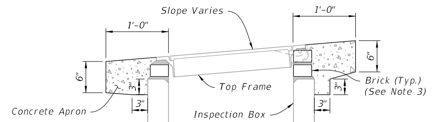
TOP ADJUSTMENT
