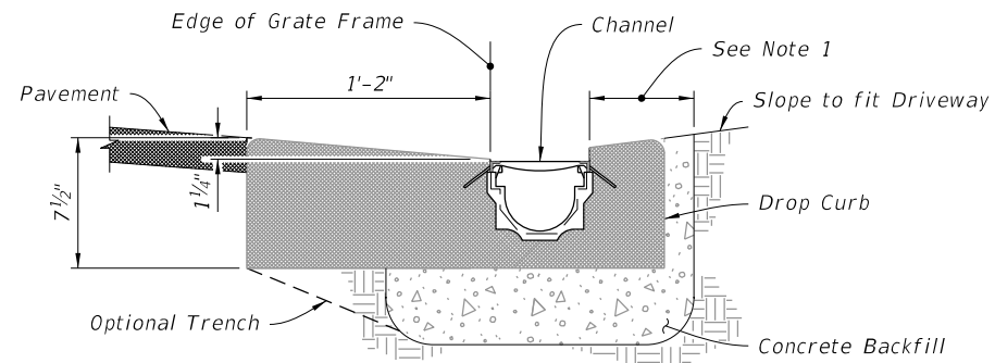
WITHIN DROP CURB
