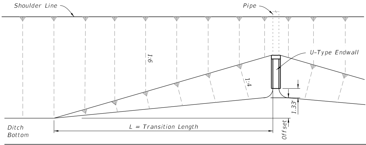
FRONT SLOPE TRANSITION AT ENDWALL
