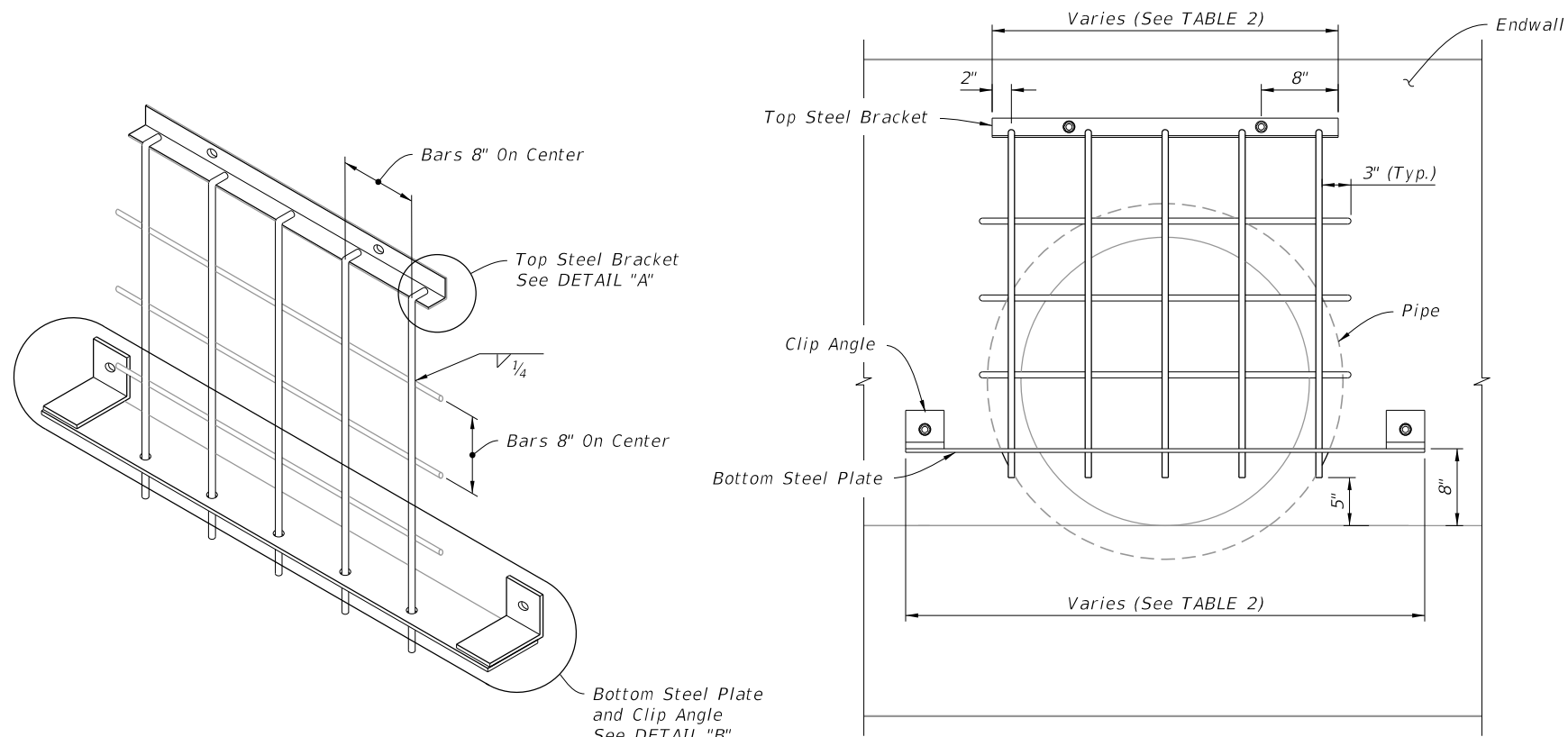
ISOMETRIC VIEW
