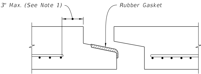
PROFILE RUBBER GASKET
