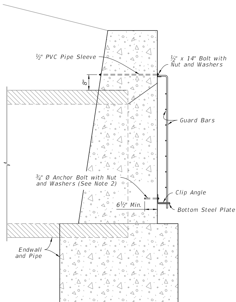
SIDE ELEVATION
