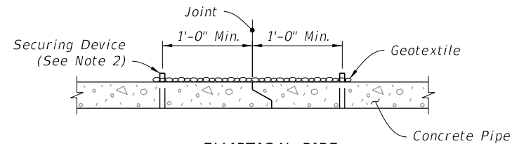
ELLIPTICAL PIPE (Tongue & Groove Shown)
