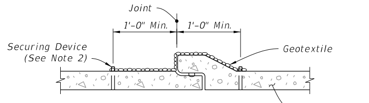
ROUND PIPE (Bell & Spigot Shown)
