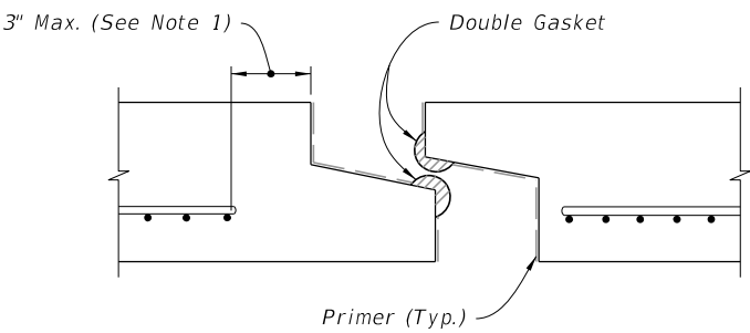
PREFORMED PLASTIC JOINT
