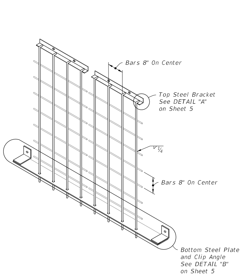
ISOMETRIC VIEW
