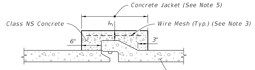
ROUND PIPE (Bell & Spigot Shown)
