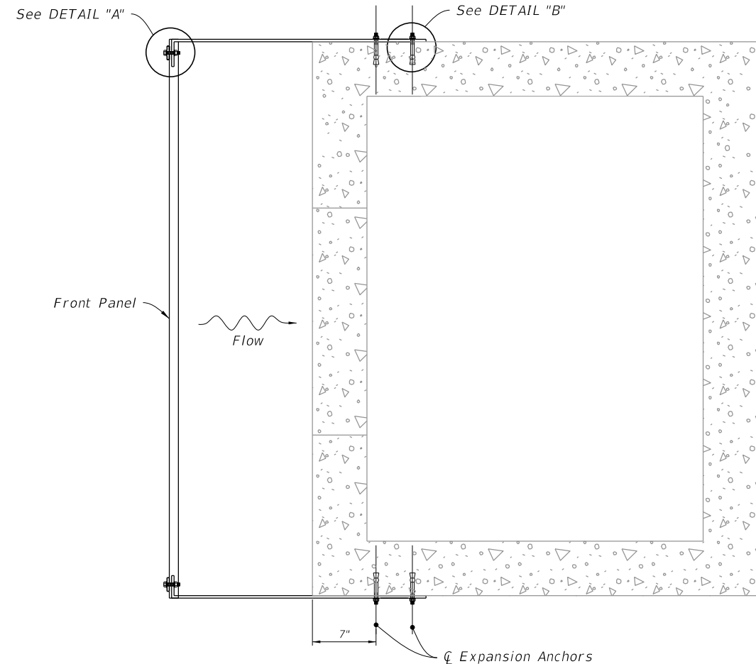
PLAN
