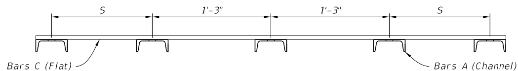
SECTION B-B
