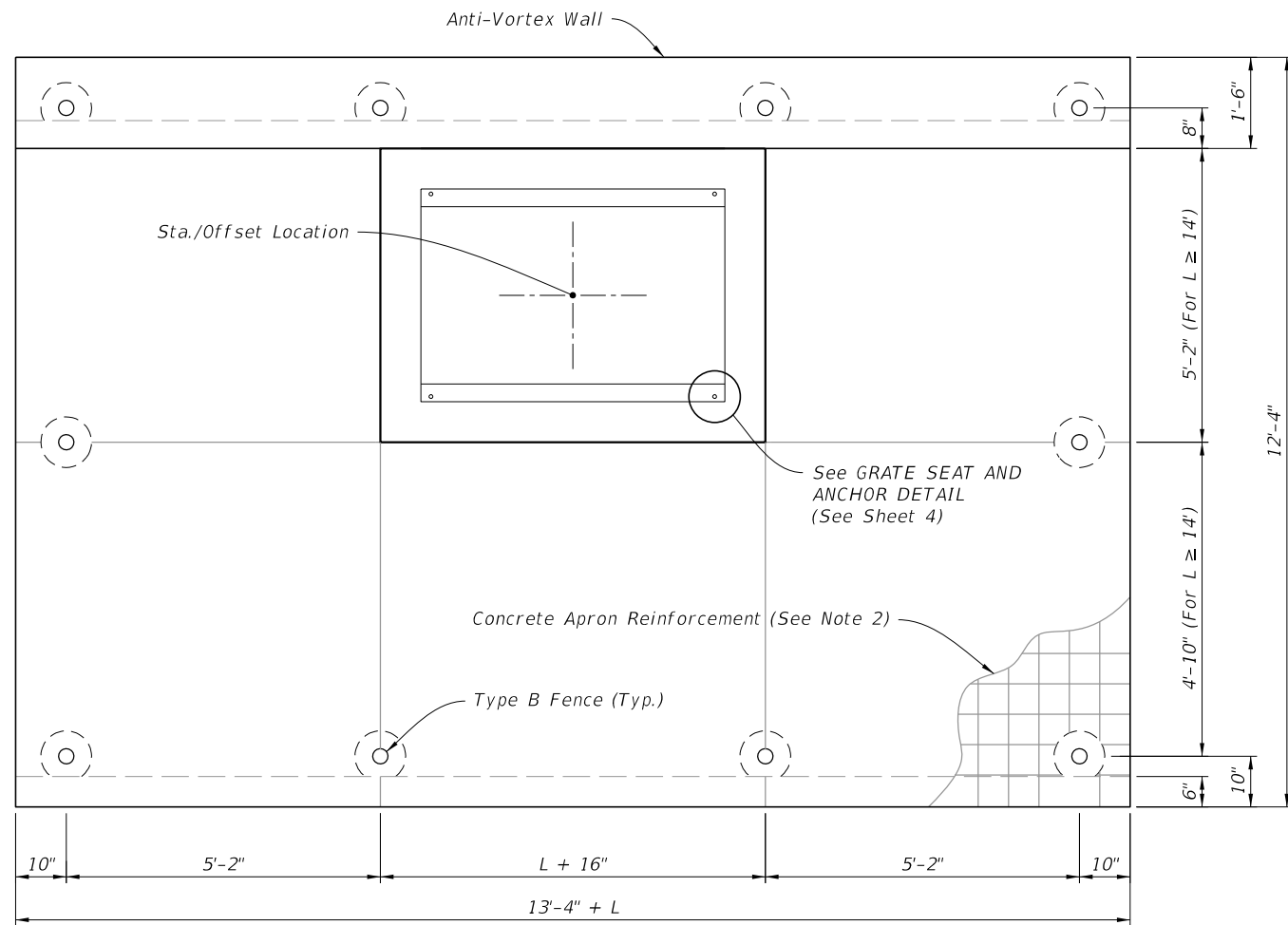
PLAN
