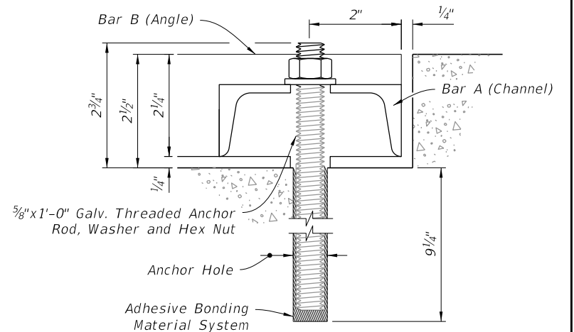
SECTION C-C
