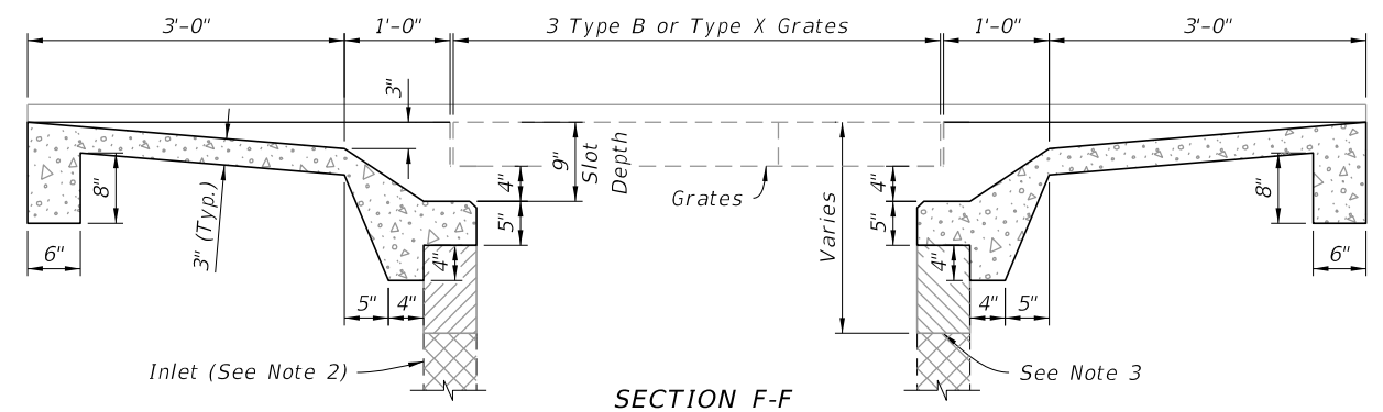
SECTION F-F
