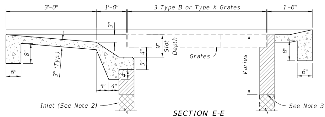
SECTION E-E
