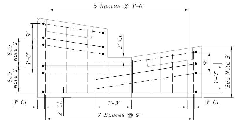
SECTION G-G
