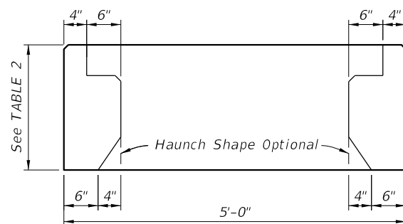
SECTION F-F
