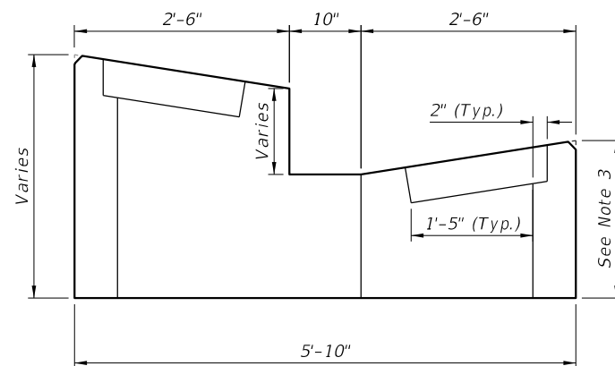
SECTION G-G
