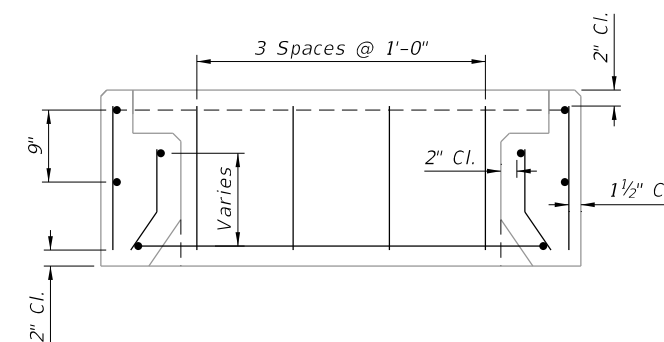
SECTION F-F
