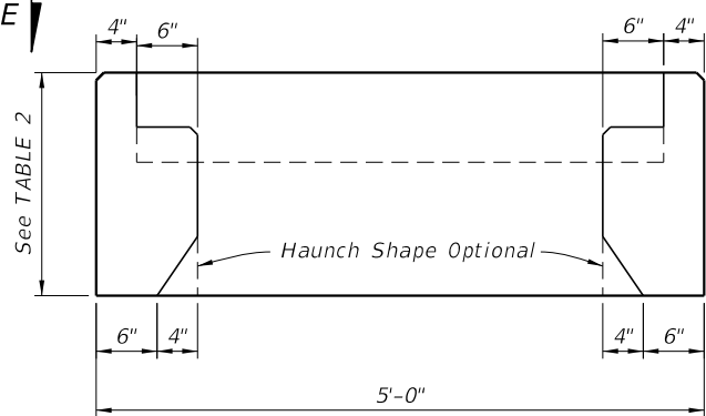
VIEW E-E
