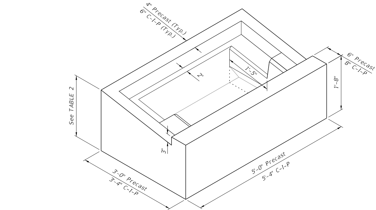
ISOMETRIC VIEW (Grate Not Shown)
