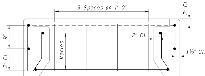
VIEW E-E
