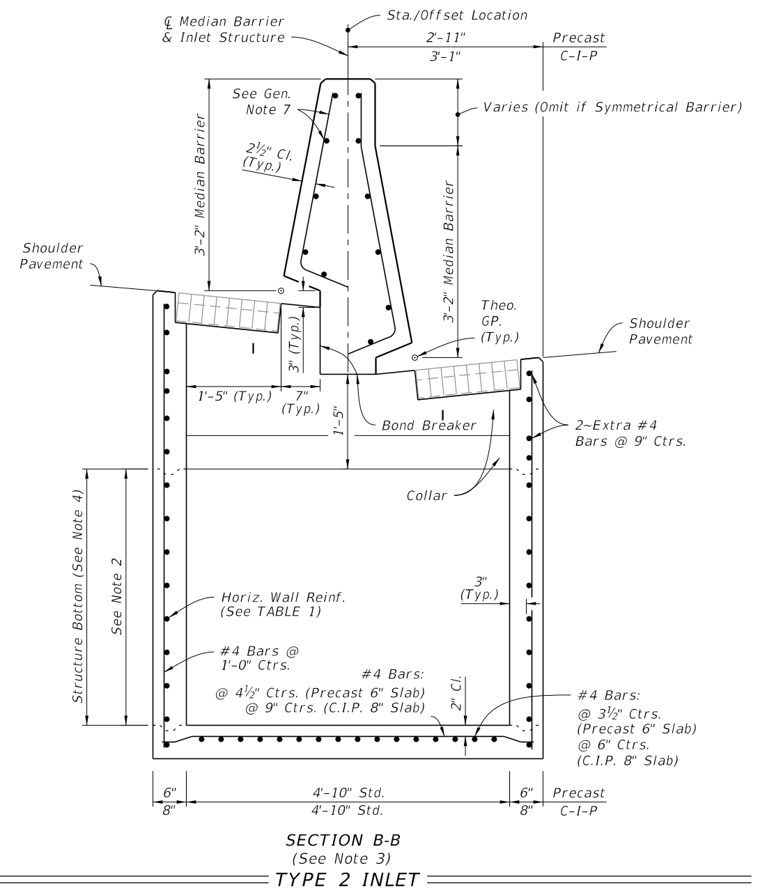
TYPE 1 AND 2 DIMENSIONAL AND REINFORCING DETAILS
