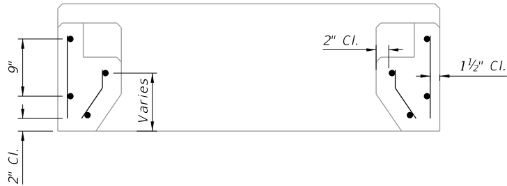
SECTION C-C
