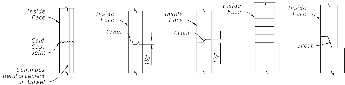
WALL JOINTS
