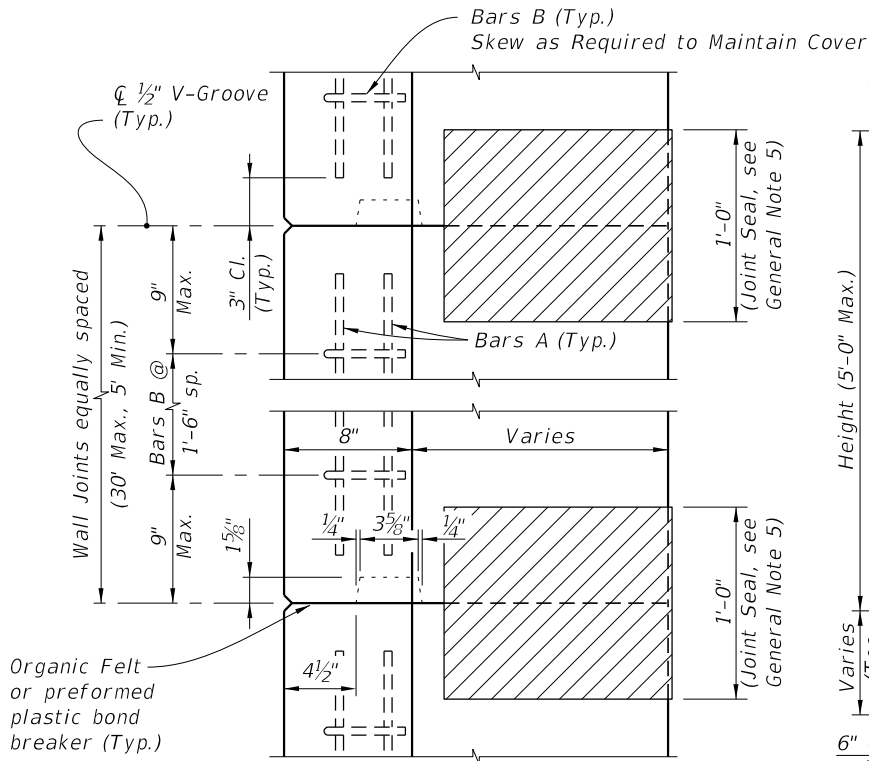
KEYWAY & WALL JOINT DETAIL (TOP VIEW)
