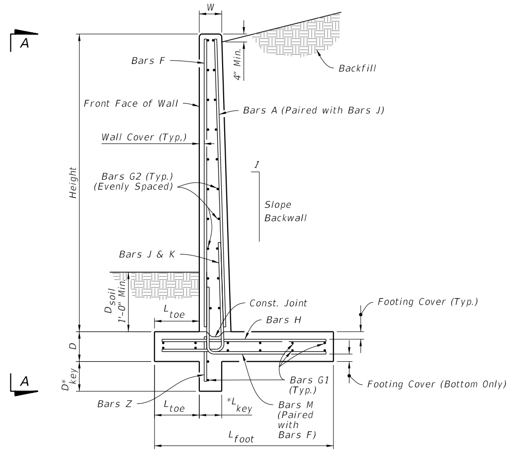
TYPICAL SECTION
