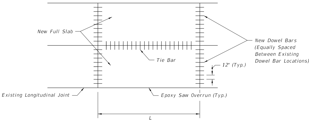
FIGURE 5 - MULTIPLE SLAB FULL DEPTH REPLACEMENT
