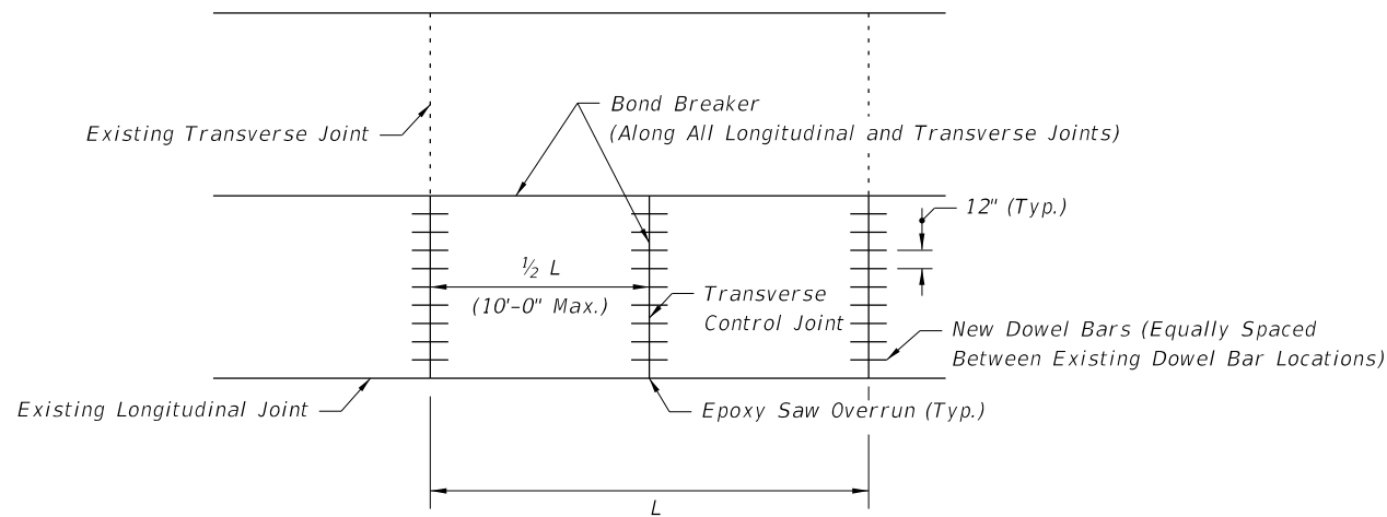
FIGURE 2 - FULL SLAB FULL DEPTH REPLACEMENT
