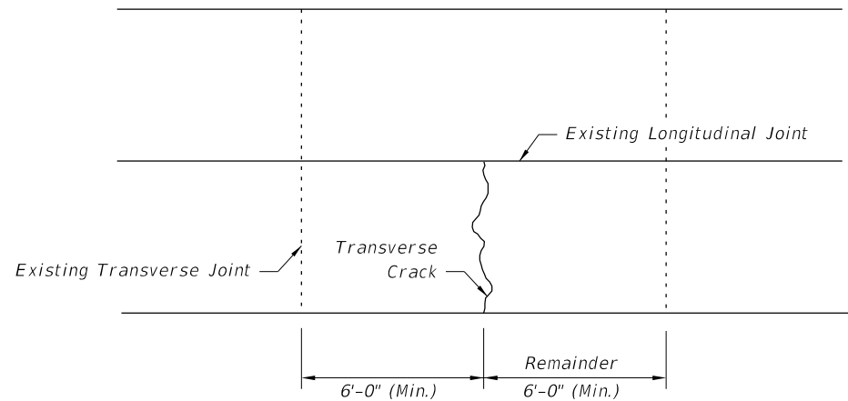
FIGURE 1 - REPAIR METHOD: NONE OR CLEAN AND SEAL
