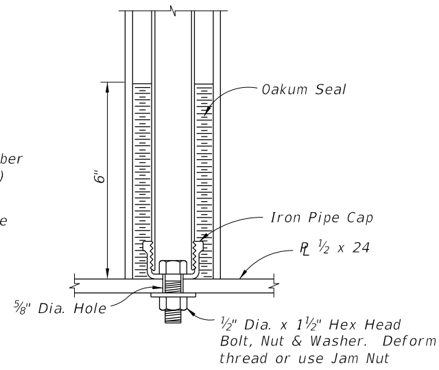
STEEL PLATE
