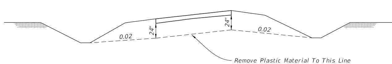
TYPICAL CUT SECTION ON SUPERELEVATION
