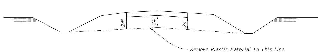
TYPICAL CUT SECTION ON TANGENT
